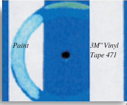
600 cycles with abrasive test wheel
